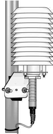
FIGURE 1. HMP45C and 41002 Radiation Shield on a CM6/CM10 Tripod Mast or UT10 Tower Leg
