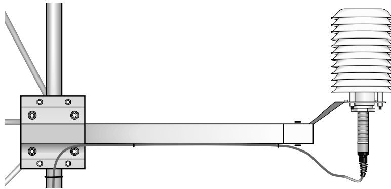
FIGURE 2. HMP45C with UT018 Mounting Bracket and Crossarm and UT12VA Radiation Shield Mounted on a UT30 Tower
