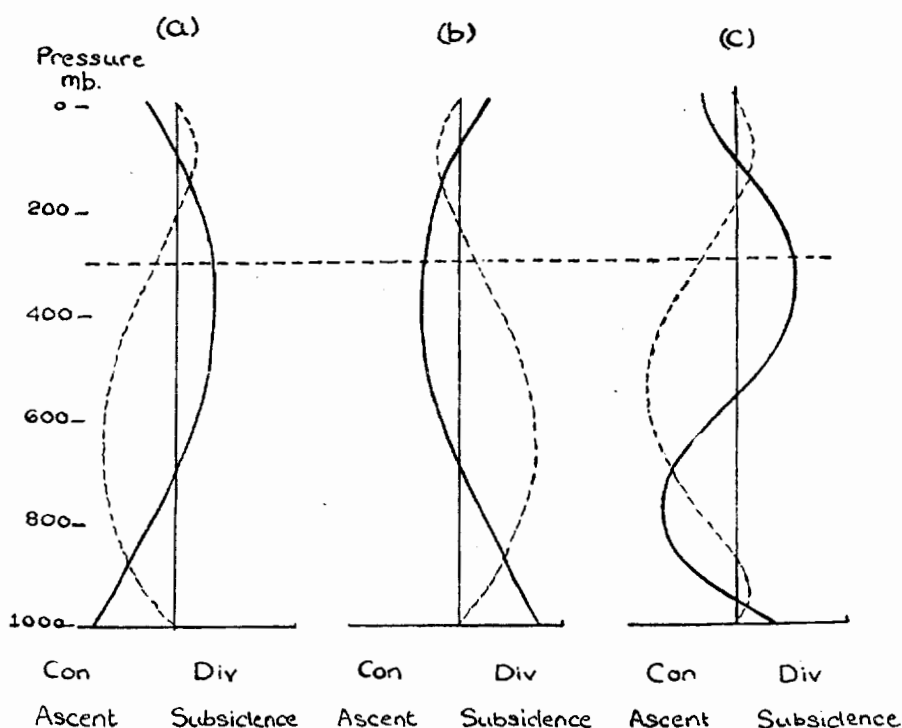
FIG. 1.—Schematic representation of the distribution with height of the isobaric divergence (full lines) and of dp/dt (broken lines).
