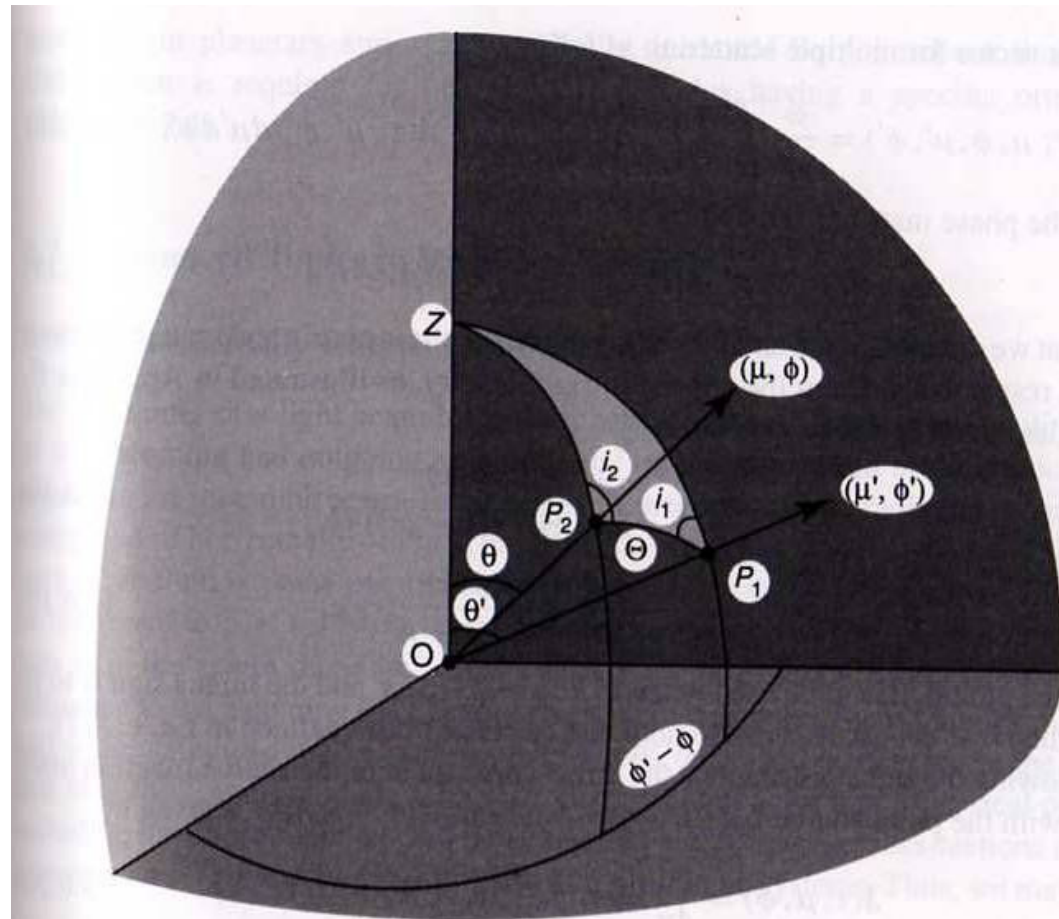
Figure 6.16 Scattering plane OP_1P_2 with respect to the meridian planes OP_1Z and OP_2Z (see the definitions of the angles).
