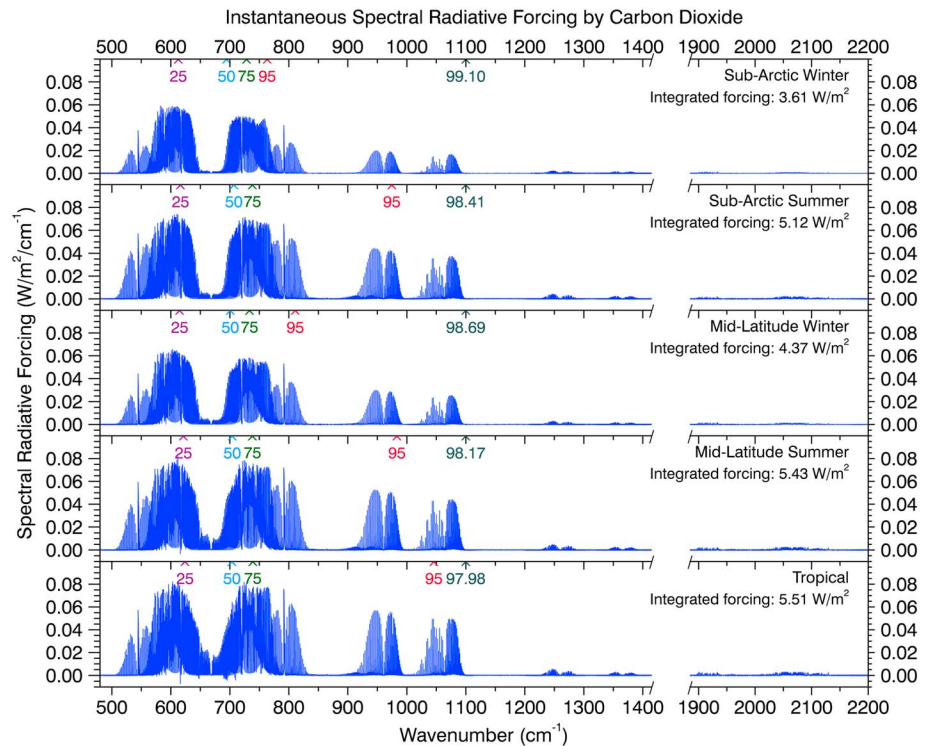
Figure 1. Spectra of instantaneous RF for doubled CO 2 (280 ppm to 560 ppm) for five different standard atmospheres. Percentiles of forcing integrating from 480 cm -1 are indicated as a function of wave number at the top of each panel. The integrated percentile to 1100 cm -1 is also indicated.
